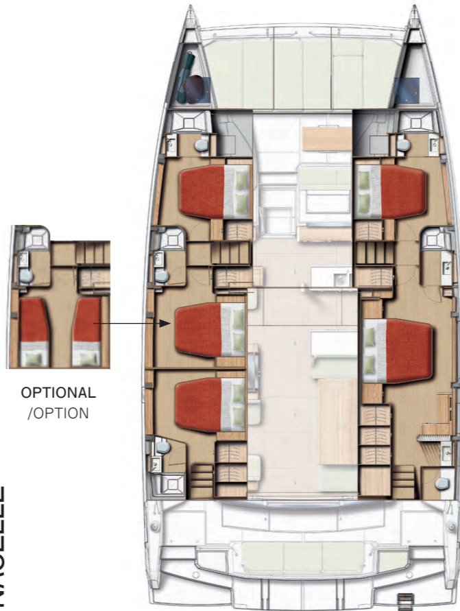
5 DOUBLE CABINS / 5 BATHS Version 5 cabines doubles / 5 sdb
